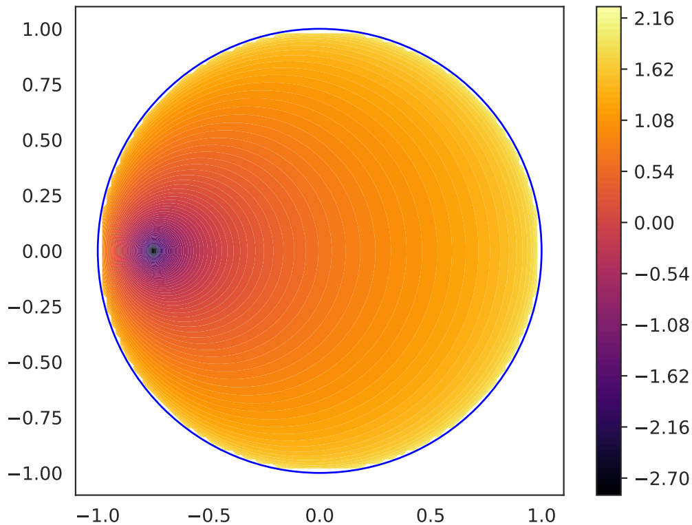
log distance to (-0.75, 0)
