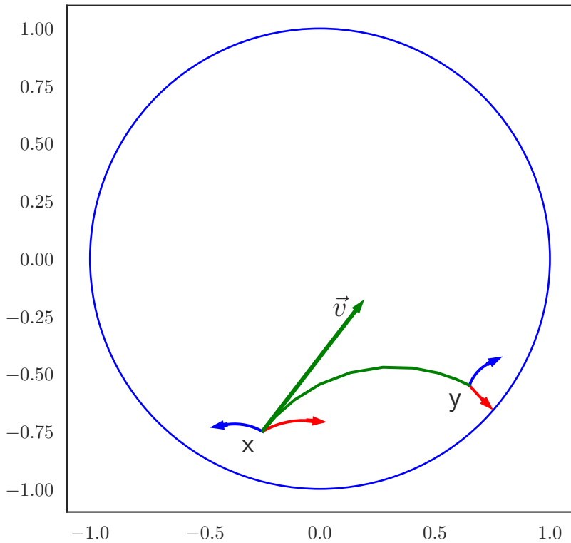
gyrovector parallel transport P_{x \rightarrow y}
